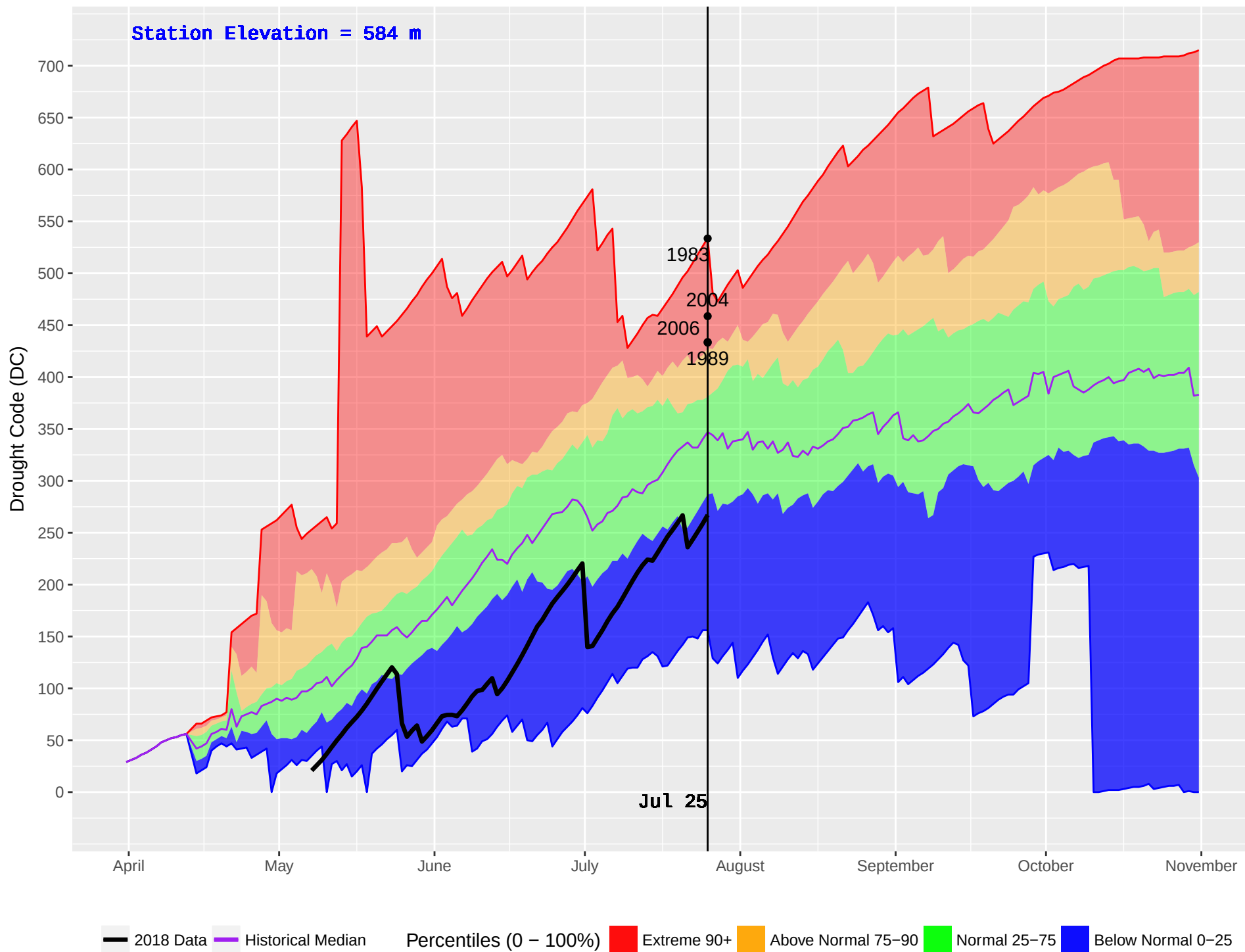
SIERRA (117) : Historical (1981–2016) and Current (2018) Noon Drought Code (DC)
