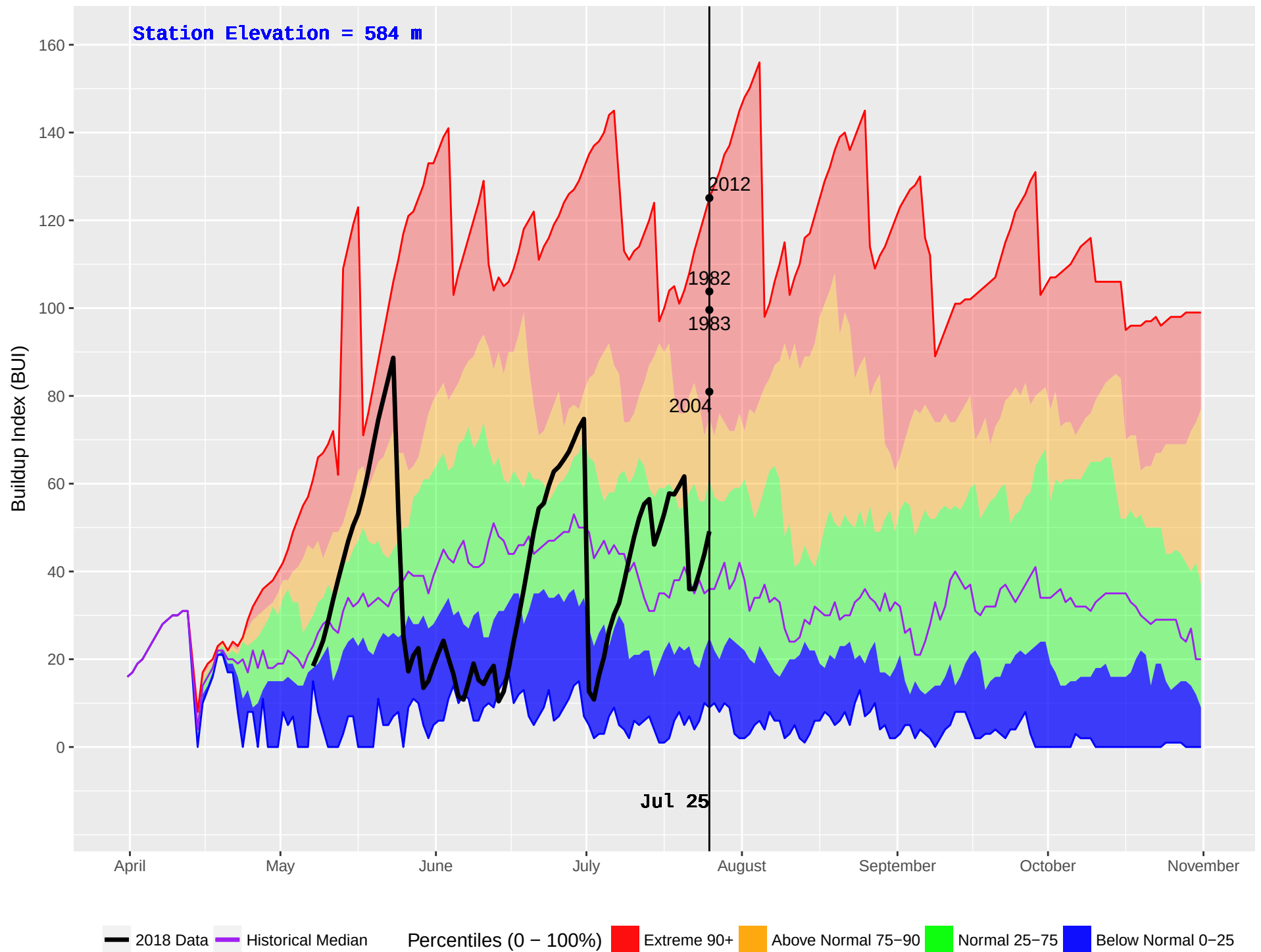
SIERRA (117) : Historical (1981–2016) and Current (2018) Noon Buildup Index (BUI)
